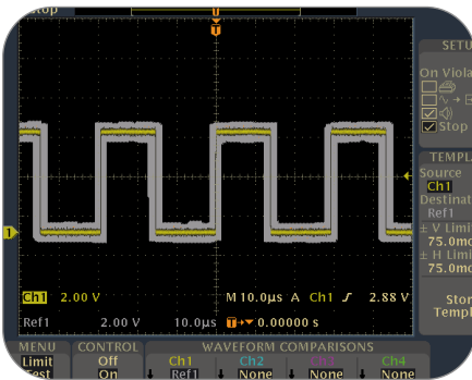
► The TDS3000B DPO with the TDS3LIM limit testing module is ideal for manufacturing test applications where fast Go/No-Go decisions are required.
