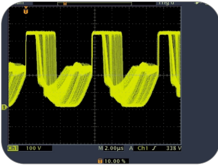
► DPO technology shows modulation effects on a power supply control loop.
